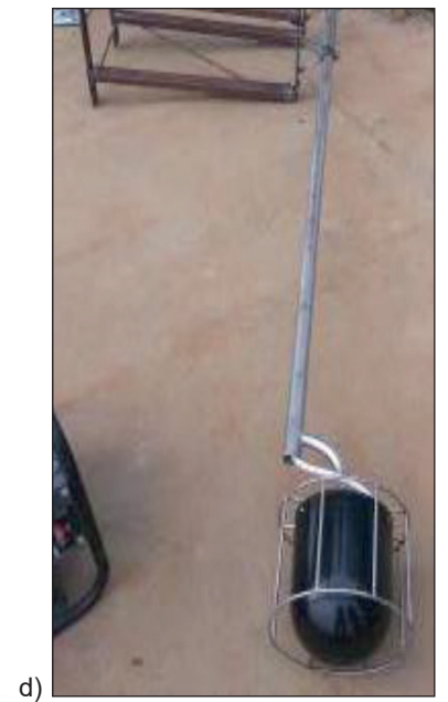
Fig. 8. General idea of the system operation (a); diagram of the sonar holder (b): 1 – sonar, 2 – temperature and pressure sensor, 3 – sonar cover, 4 – holder, 5 – holder mounting, 6 – power and data cable; rotating mechanism (c); sonar with holder (d); →
