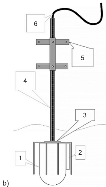
Fig. 8. General idea of the system operation (a); diagram of the sonar holder (b): 1 – sonar, 2 – temperature and pressure sensor, 3 – sonar cover, 4 – holder, 5 – holder mounting, 6 – power and data cable; rotating mechanism (c); sonar with holder (d); →
