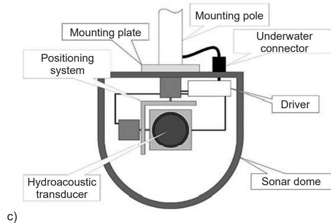
Fig. 8. General idea of the system operation (a); diagram of the sonar holder (b): 1 – sonar, 2 – temperature and pressure sensor, 3 – sonar cover, 4 – holder, 5 – holder mounting, 6 – power and data cable; rotating mechanism (c); sonar with holder (d); →
